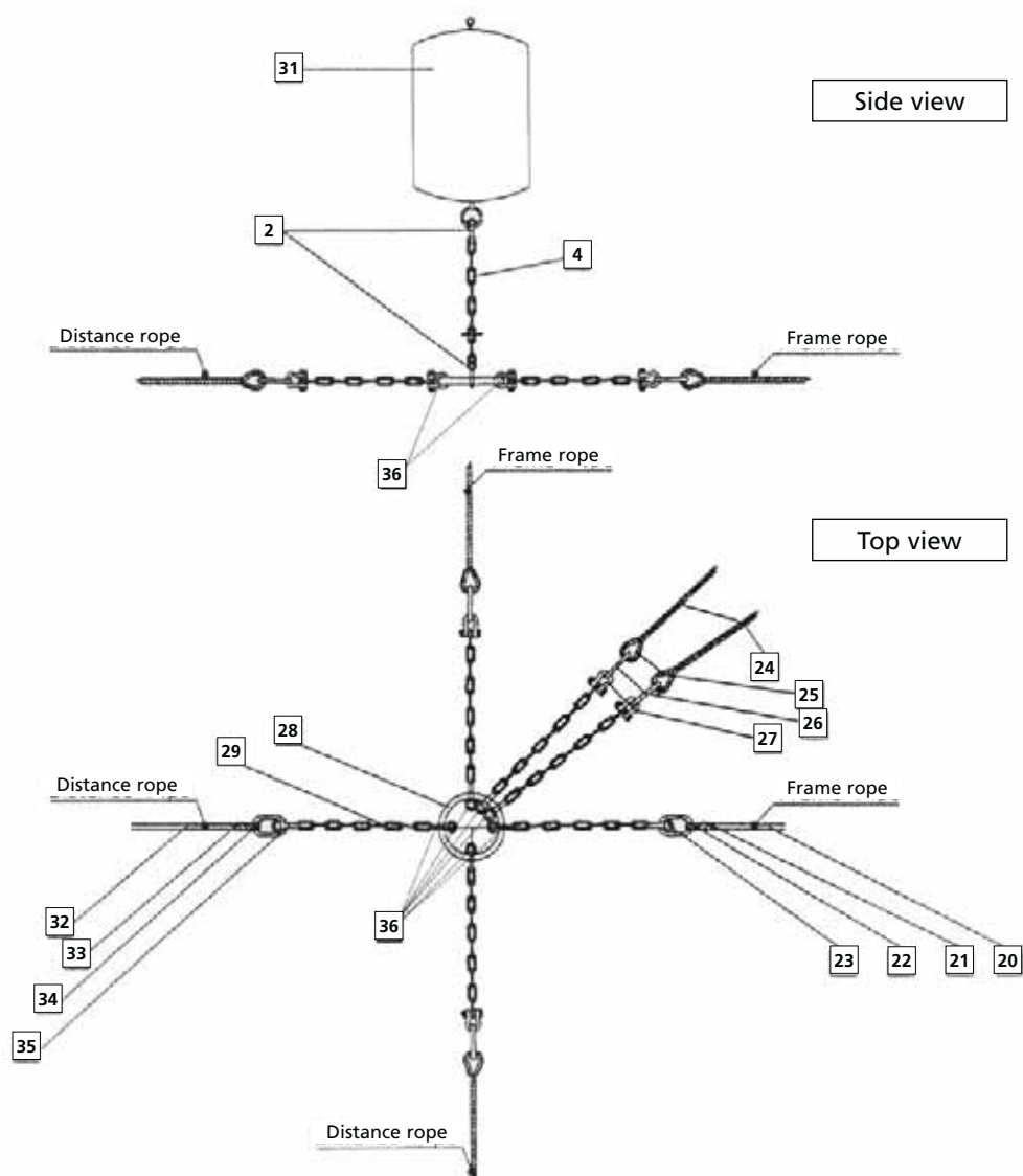
FIGURE A1.3 Corner connection
