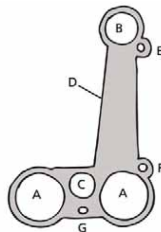
FIGURE 29 Standard bracket scheme (two floating pipes, side elevation)
